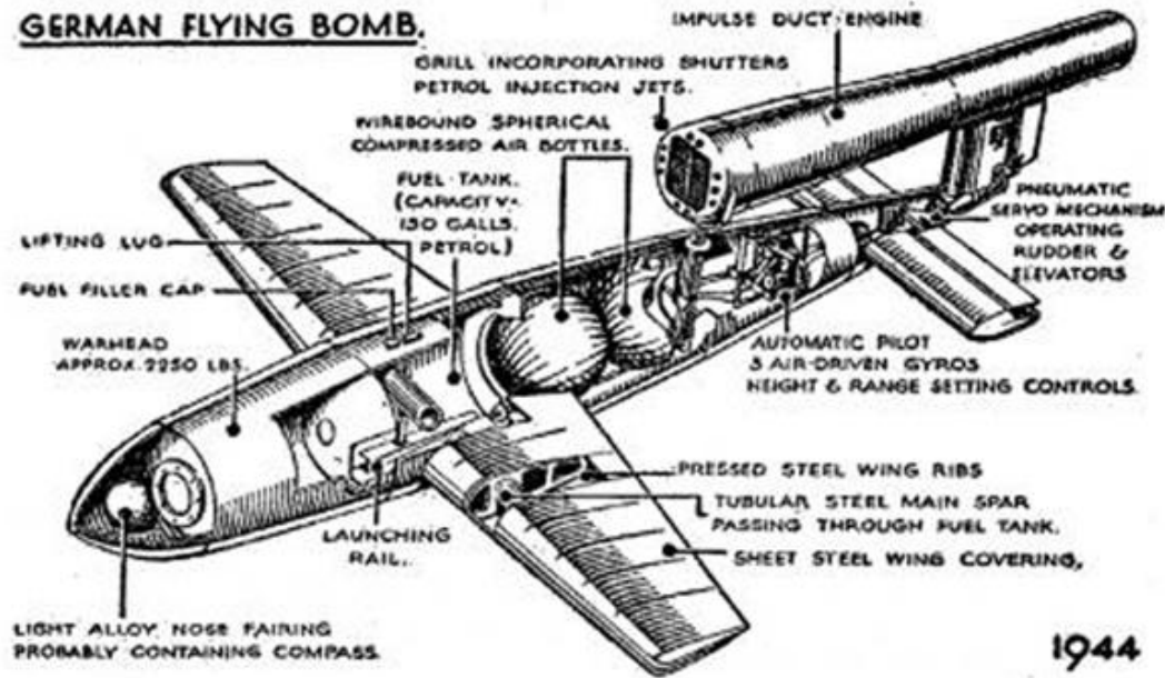
FLYING BOMB F.Z.G. 76
